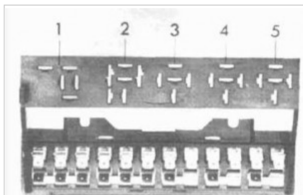
Volkswagen Beetle (1954 – 1979) – fuse box
